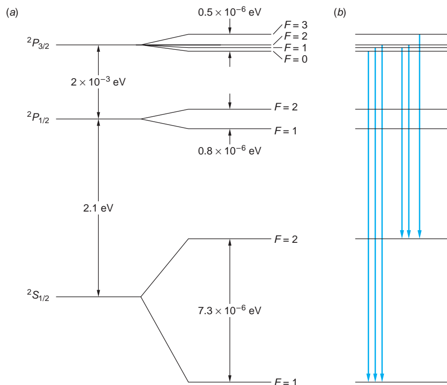
FIGURE 11-11 (a) Transitions between the sodium doublet levels produce the yellow D lines, 2P_{1/2} \rightarrow 2S_{1/2} being D_1 and 2P_{3/2} \rightarrow 2S_{1/2} being D_2 . Coupling between the atomic angular momentum J and the nuclear spin I = 3/2 results in the hyperfine splitting, each level having total angular momentum \mathbf{F} = \mathbf{I} + \mathbf{J} . Note that the hyperfine splitting of each of the doublet levels is about 10^{-3} times that of the fine-structure splitting of the 2P level. (b) The selection rule \Delta F = \pm 1, 0 leads to the D_2 line being split into six components. The D_1 line is correspondingly split into four components (not shown).
